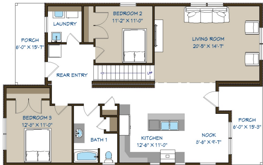
1 ST FLOOR – 1492 SQ FT
